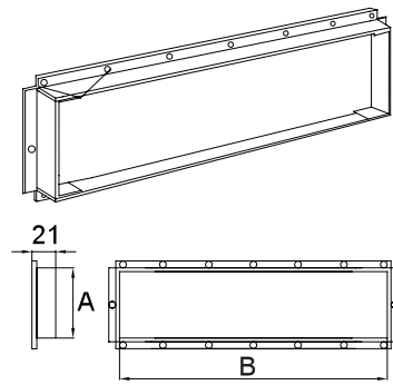
Fig.9 Air Supply Outlet
